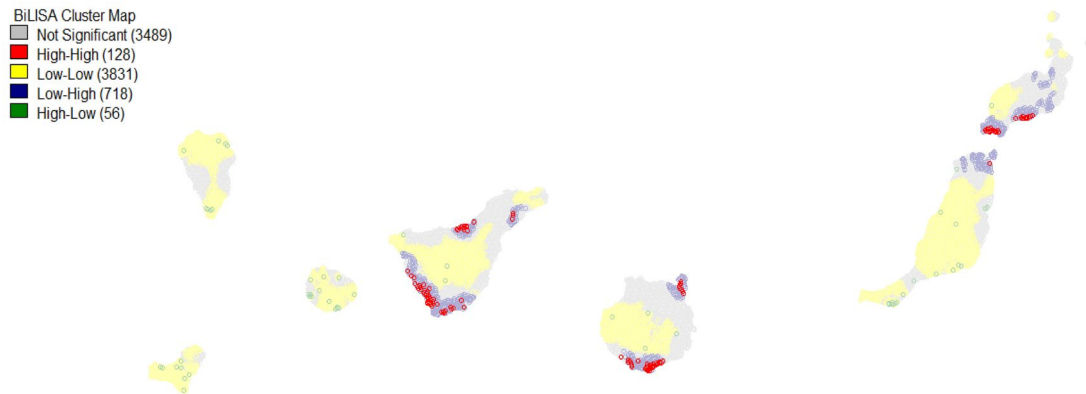
Figure 3. Figure 3. Bivariate LISA clustering of established hotels and Airbnb spatial correlation (80NN spatial weight matrix)
